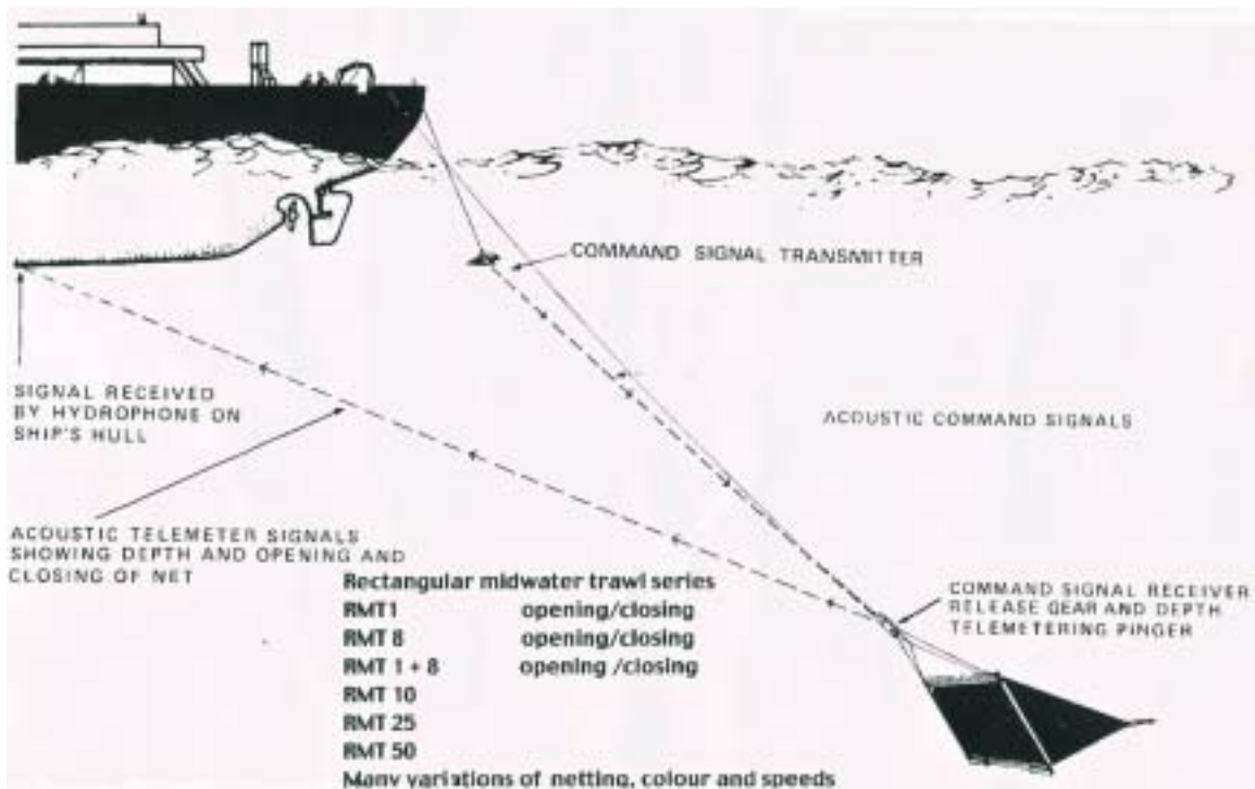
Figure 5. The rectangular midwater trawls designed to sample a large size range of animals while fishing in the same way as well as opening and closing to study vertical distribution.
