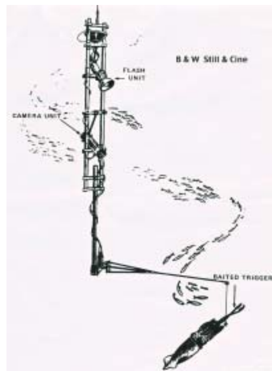
Figure 2. The baited still camera used to photograph deep sea squids.
