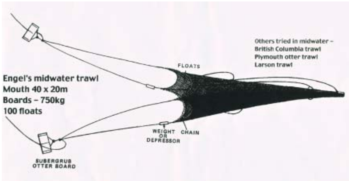
Figure 4. The large Engel's otter trawl.
