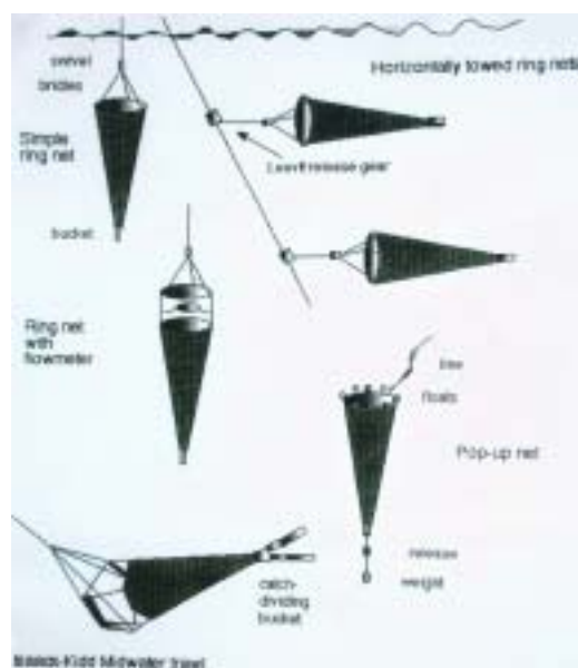
Figure 3. Ring nets used in 1959–64, a pop-up net and an Isaacs-Kidd midwater trawl.
